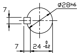
OUTPUT SHAFT
